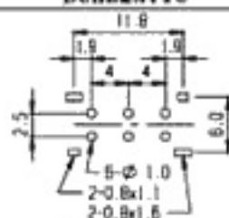
PCB LAYOUT
